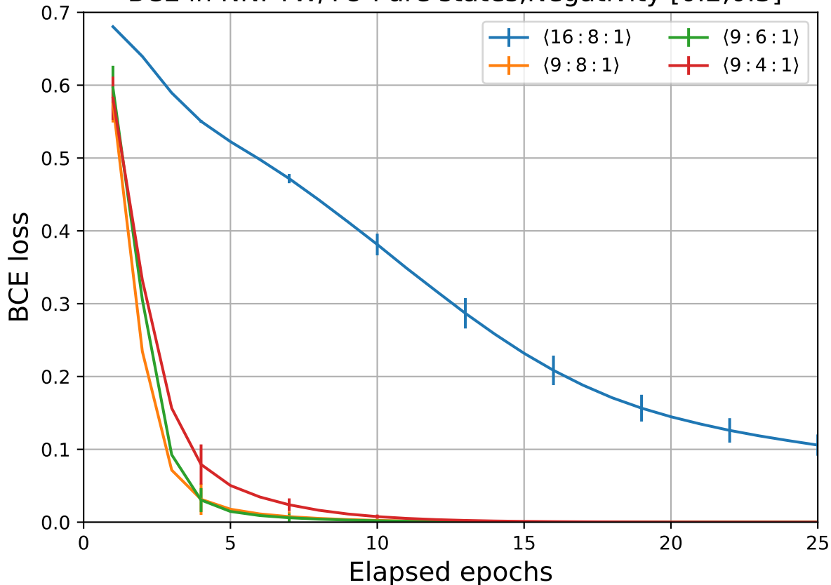
BCE in NN. TW/TO Pure states, Negativity [0.2,0.3]
