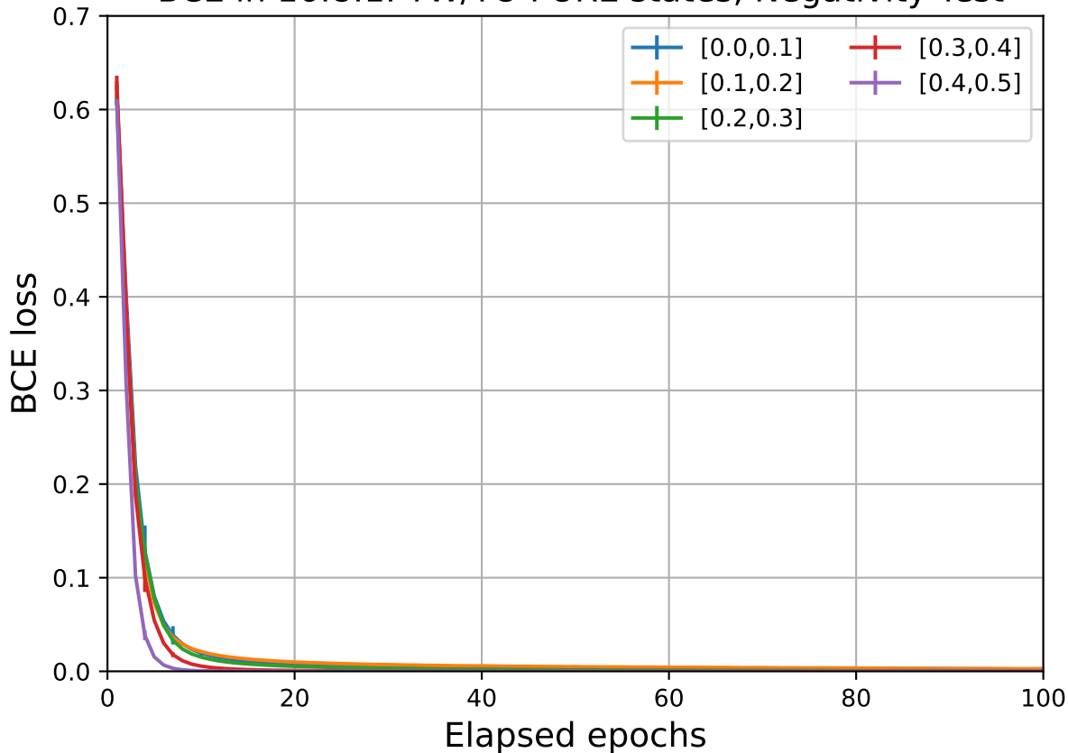
BCE in 16:8:1. TW/TO PURE states, Negativity Test
