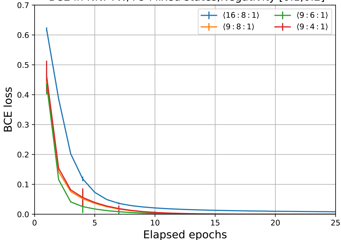
BCE in NN. TW/TO Mixed states, Negativity [0.1,0.2]
