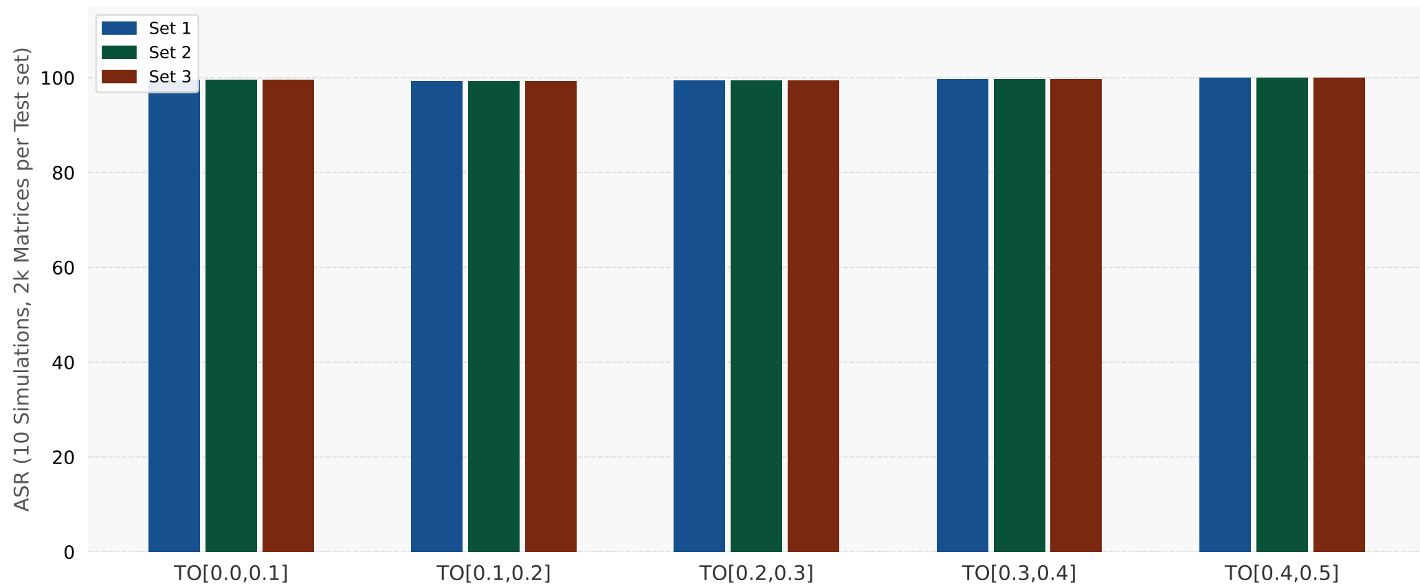
Trained Separable Mixed & Entangled Mixed [0.0, 0.1], Tested on Separable Mixed & Entangled Mixed
