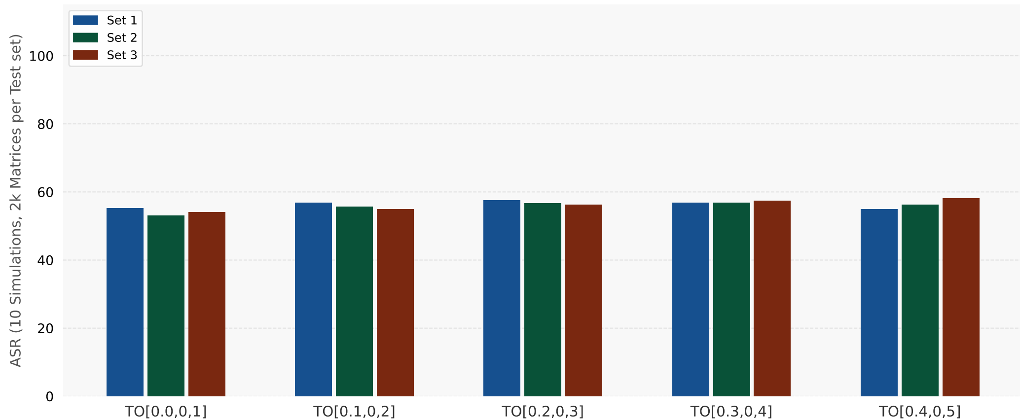
Trained with Pure Separable & Entangled in [0.0, 0.1] , Tested on Pure Separable & Entangled
