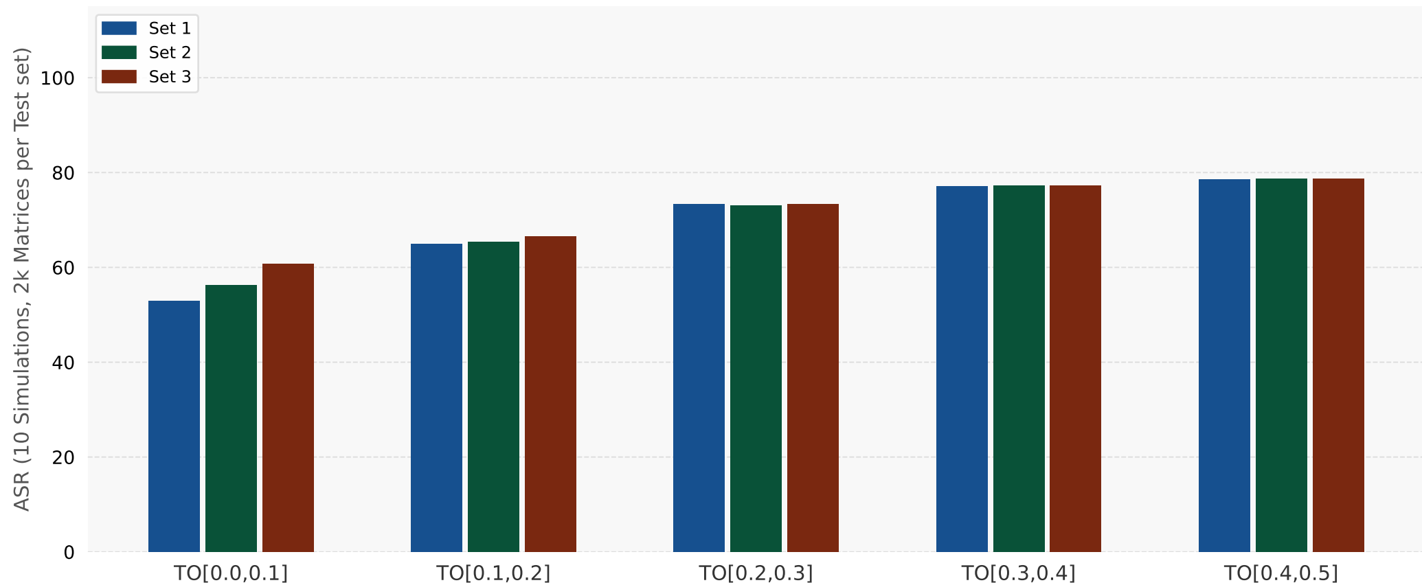
Trained with Pure Separable & Entangled in [0.2, 0.3] , Tested on Pure Separable & Entangled
