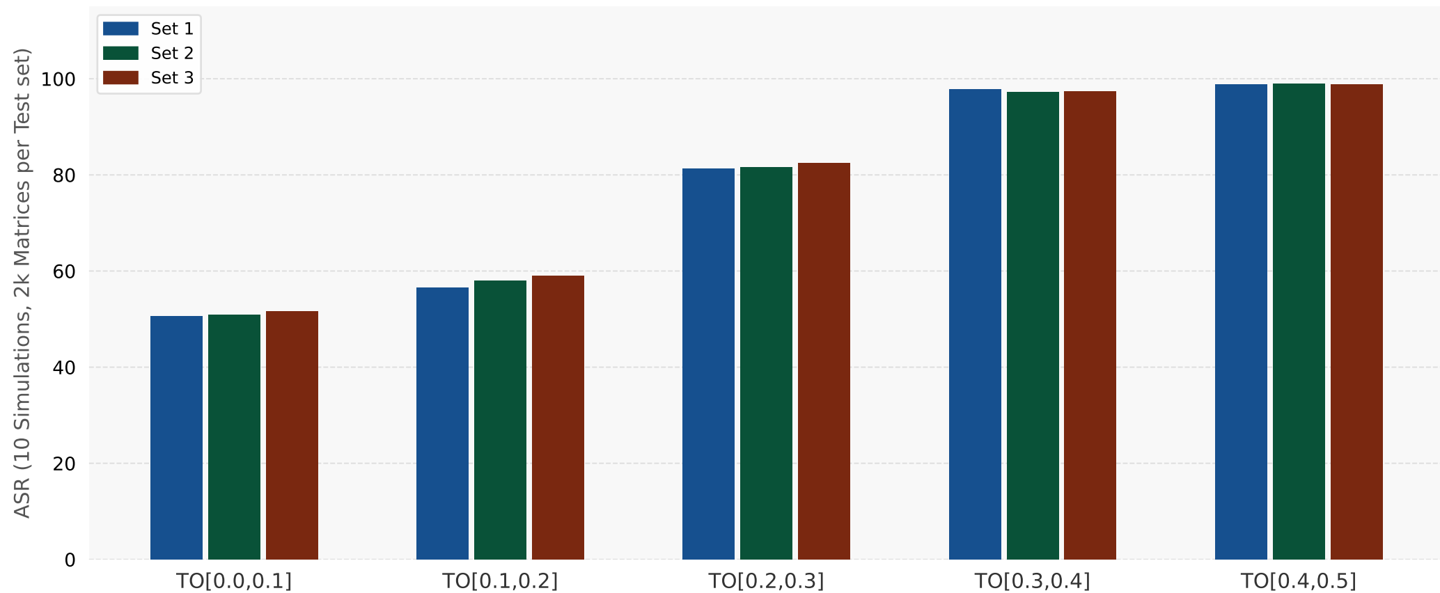
Trained with Pure Separable & Entangled in [0.4, 0.5] , Tested on Pure Separable & Entangled
