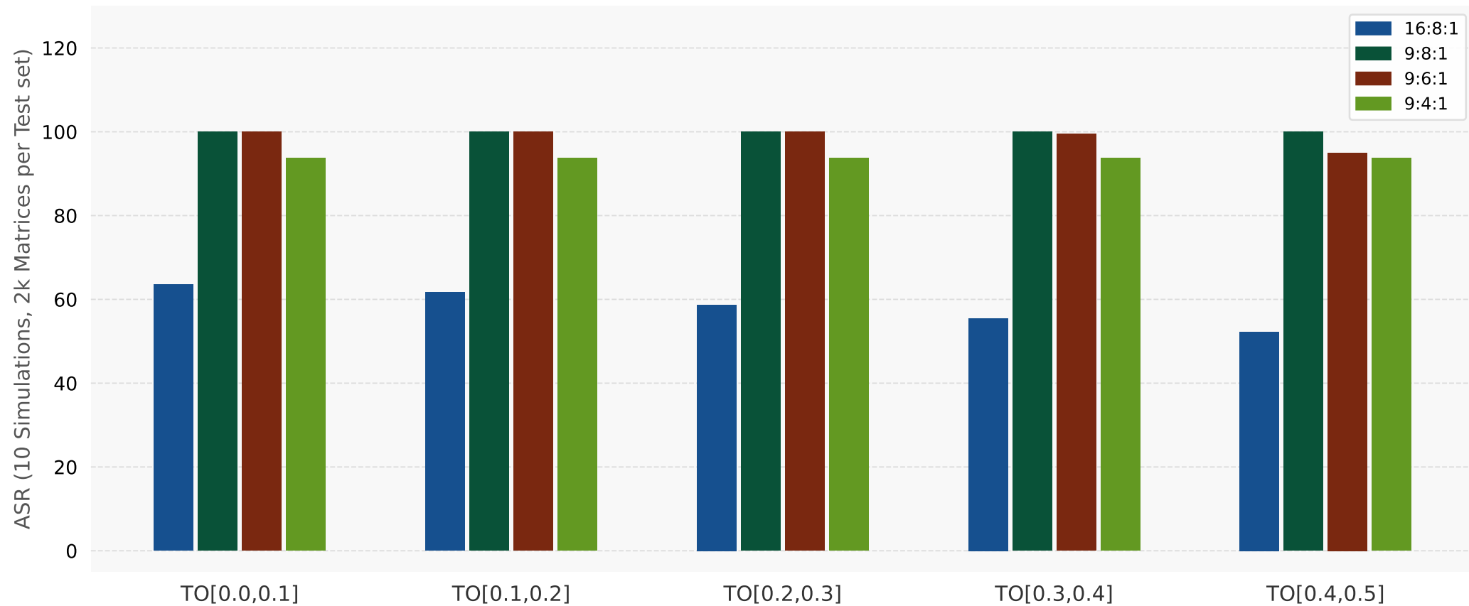
Trained with Pure Separable & Entangled in [0.0, 0.1] , Tested on Mixed Separable & Entangled, different NN
