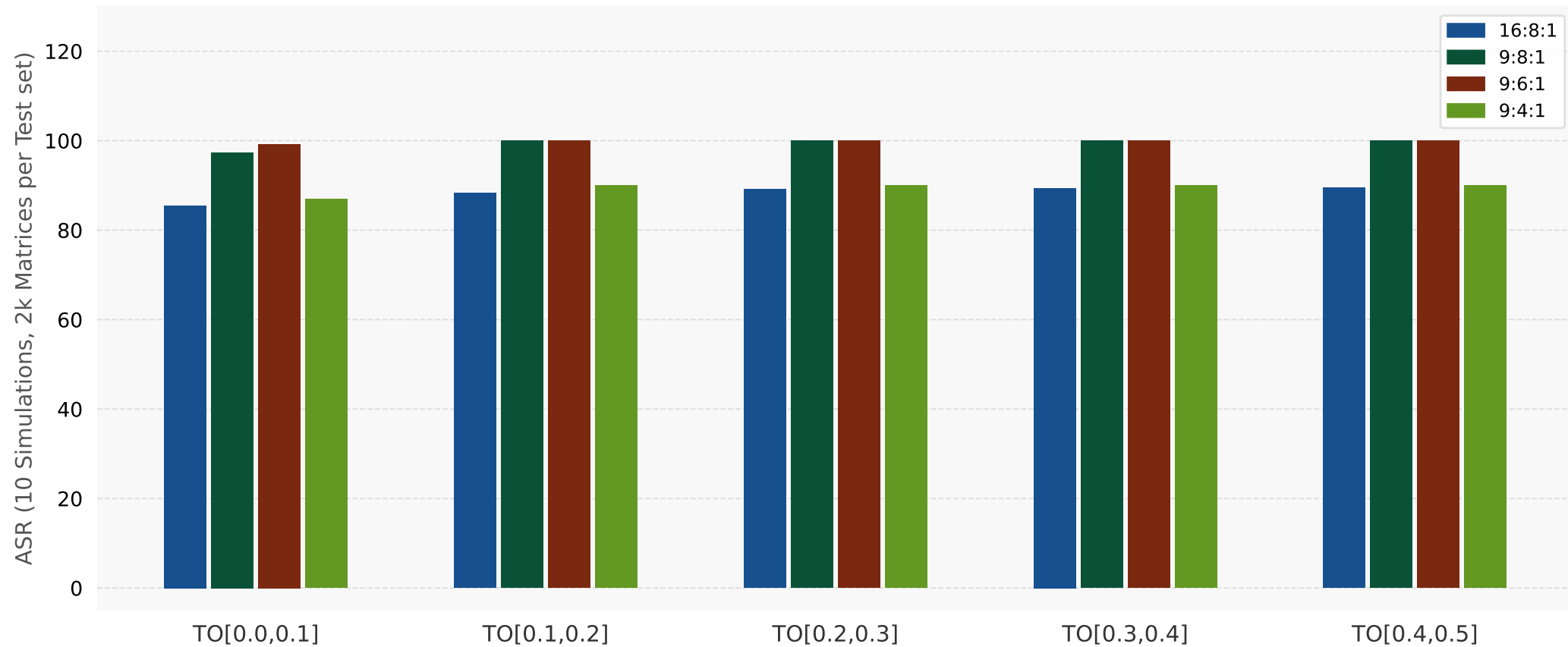
Trained with Pure Separable & Entangled in [0.2, 0.3] , Tested on Mixed Separable & Entangled, different NN
