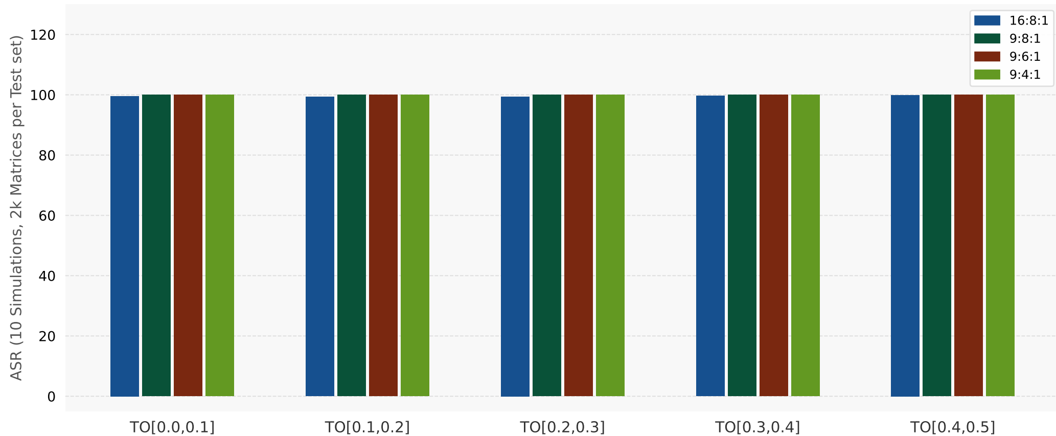
Trained with Mixed Separable & Entangled in [0.0, 0.1] , Tested on Mixed Separable & Entangled, different NN
