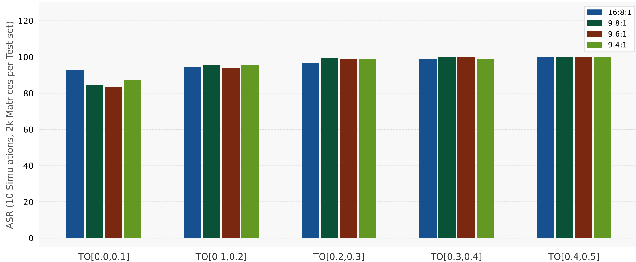
Trained with Mixed Separable & Entangled in [0.4, 0.5] , Tested on Mixed Separable & Entangled, different NN
