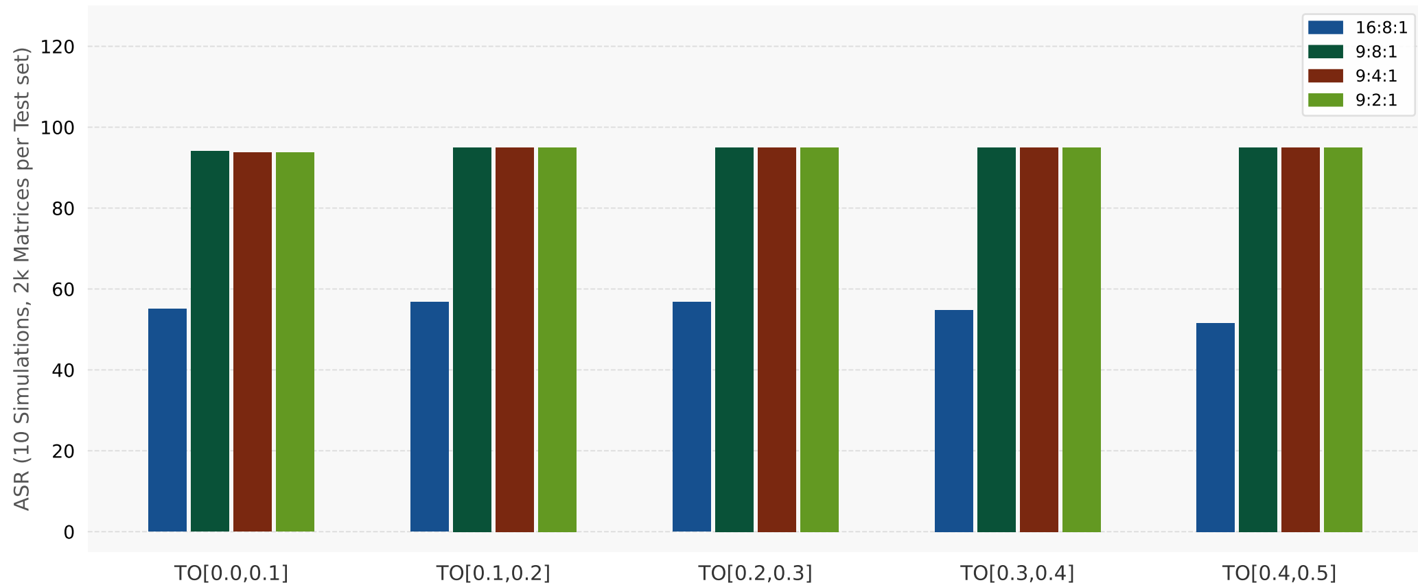
Trained with Pure Separable & Entangled in [0.0, 0.1] , Tested on Pure Separable & Entangled, different NN
