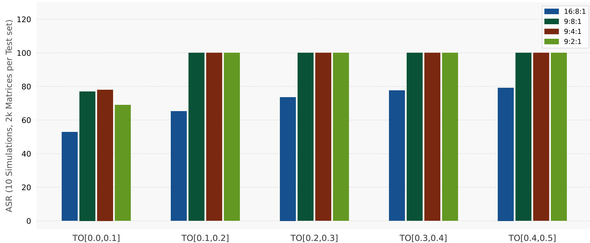
Trained with Pure Separable & Entangled in [0.1, 0.2] , Tested on Pure Separable & Entangled, different NN
