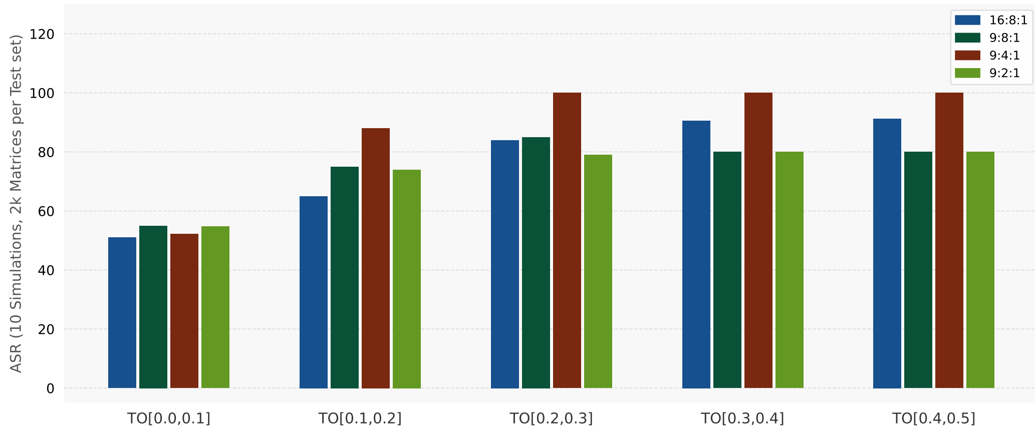
Trained with Pure Separable & Entangled in [0.2, 0.3] , Tested on Pure Separable & Entangled, different NN
