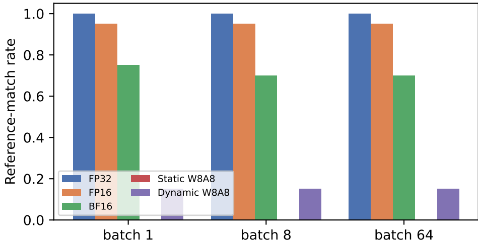
Greedy match to FP32 batch-1 reference
