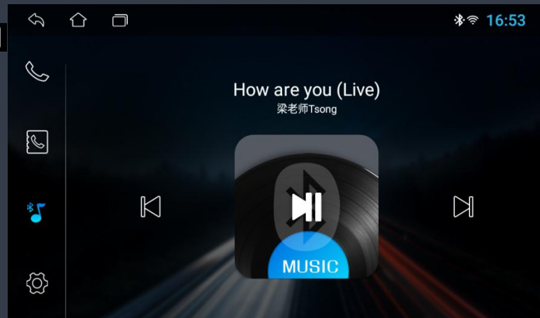
Figure 5.4 Bluetooth Music
