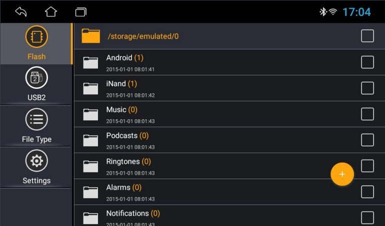
Figure 15.1 File Manager
