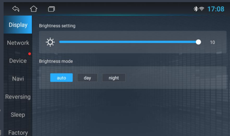
Figure 19.1 Car settings
