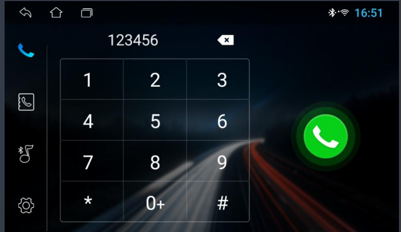
Figure 5.2 Dial-up interface
