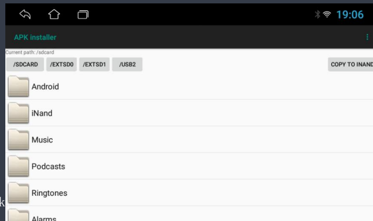
Figure 18.1 apk installer
