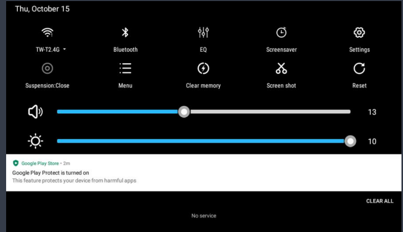
Figure 2.1 Drop-down menu
