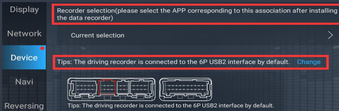
Figure 13.1 Recorder function
