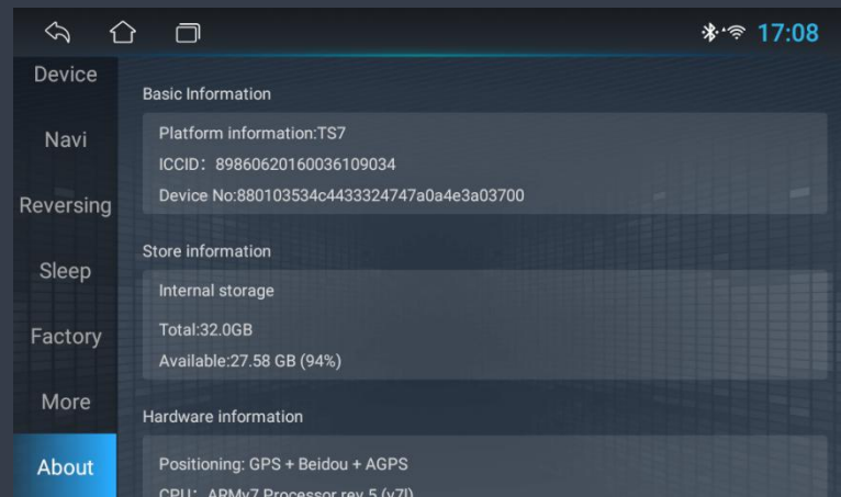
Figure 19.2 Car settings
