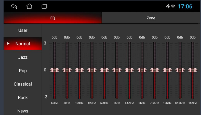
Figure 17.1 Equalizer
