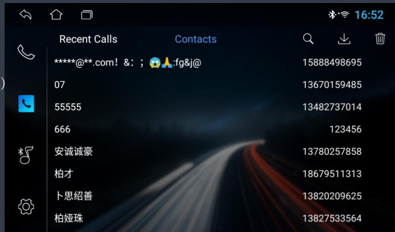
Figure 5.3 Contacts
