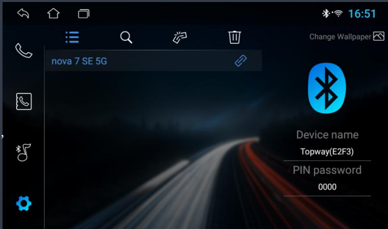
Figure 5.1 Bluetooth settings
