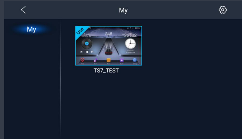
Figure 4.1 Theme
