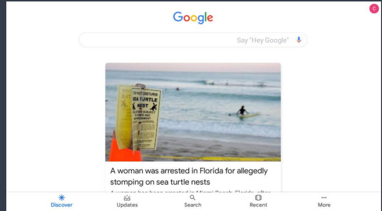
Figure 9.1 Google voice
