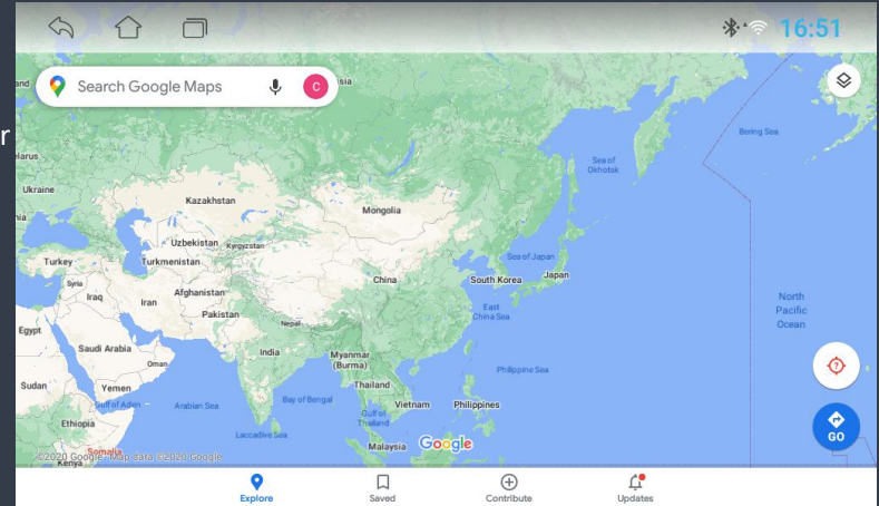
Figure 3.1 Navigation
