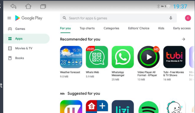
Figure 11.1 play store
