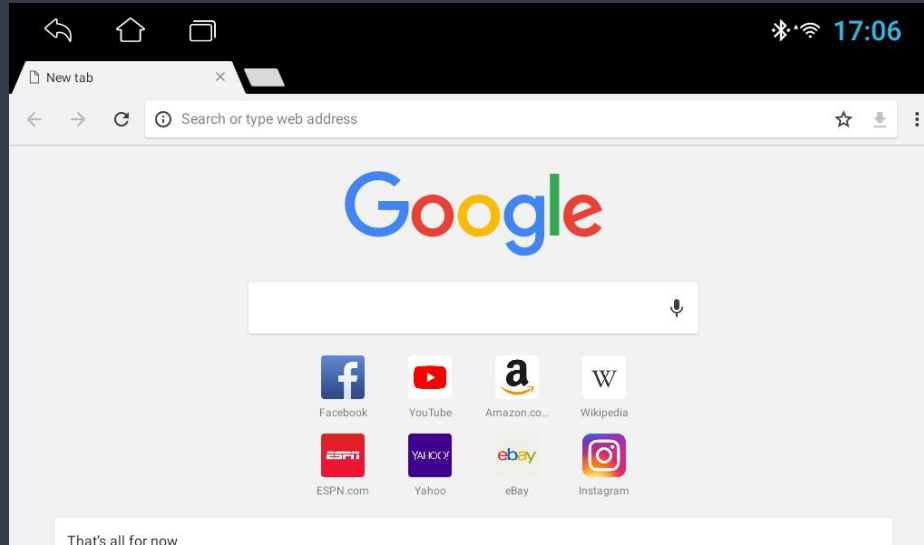
Figure 16.1 Browser
