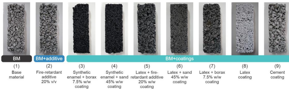
Fig. 3. Types of samples used in the single flame source test.
