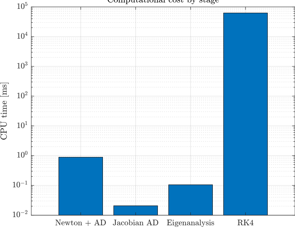
Computational cost by stage
