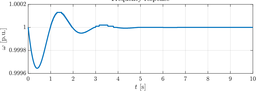
Frequency response
