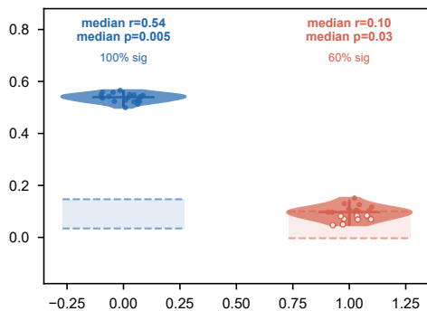
Canonical correlation
