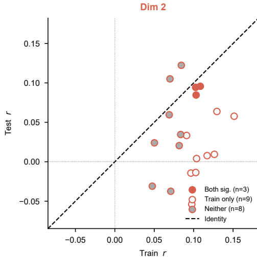
Train vs. test canonical correlation (diagonal = perfect generalisation)
