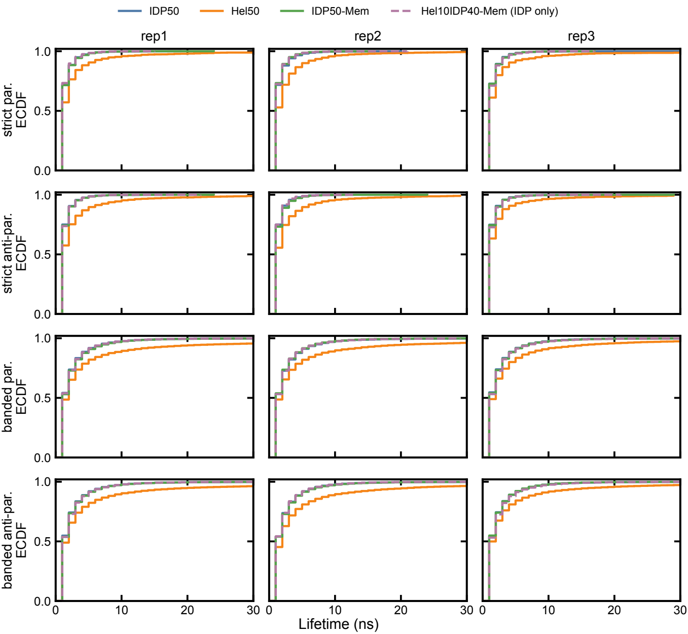
Persistent largest-cluster chains: three-consecutive ECDFs
