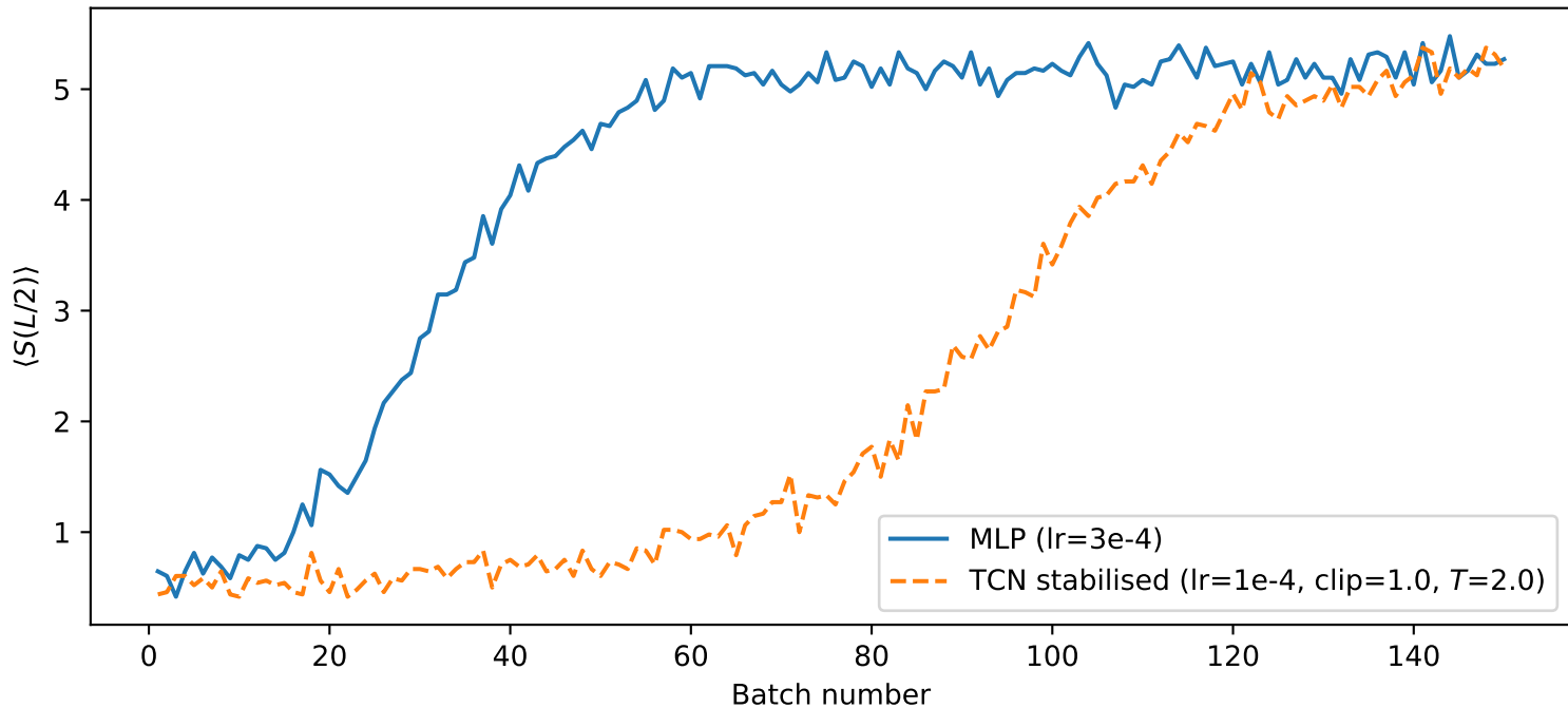
Training curves — L = 24 , k = 8 : MLP vs stabilised TCN
