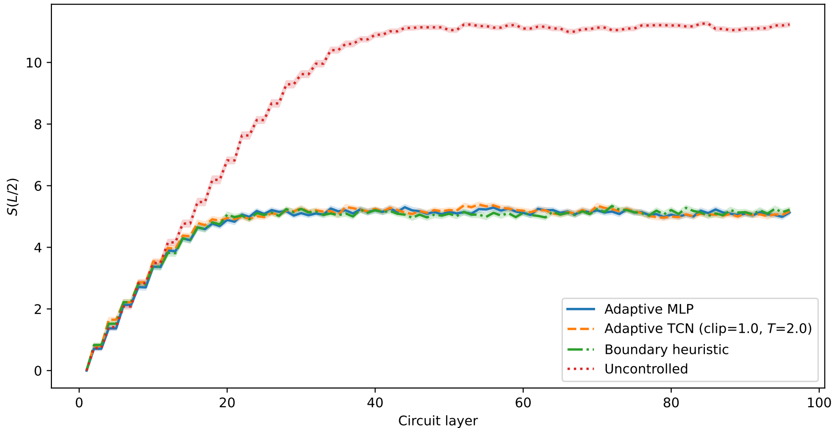
Entropy trajectory — L = 24 , k = 8 : MLP vs stabilised TCN
