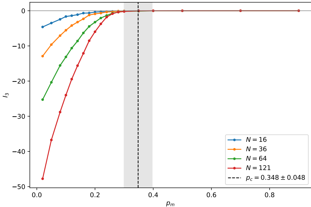
2D lattice (v2, depth = 4N) — I_3 vs measurement rate
