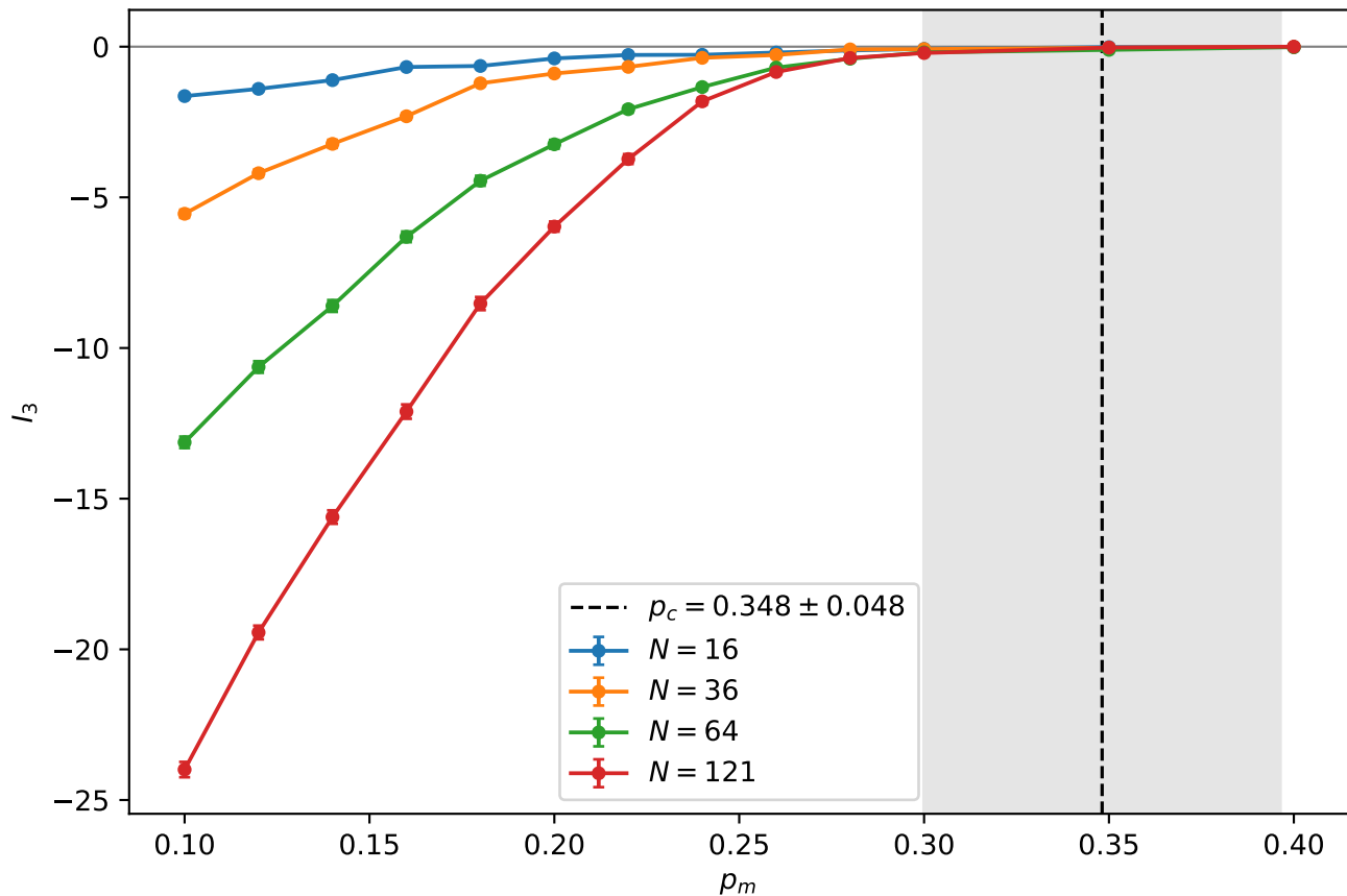
2D lattice (v2, depth = 4N) — l_3 crossing
