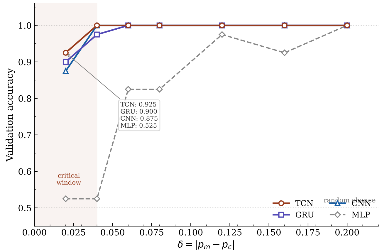
Phase classification accuracy vs \delta = |p_m - p_c| ( L = 16 )
