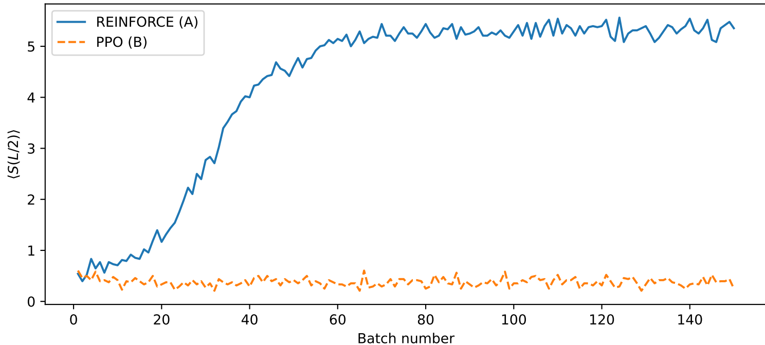
Training curves — L = 24, k = 8 : REINFORCE vs PPO
