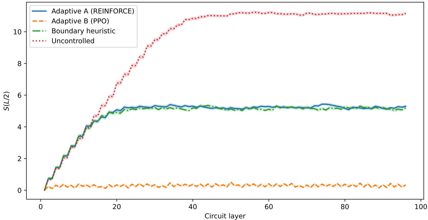
Entropy trajectory — L = 24 , k = 8 : REINFORCE vs PPO
