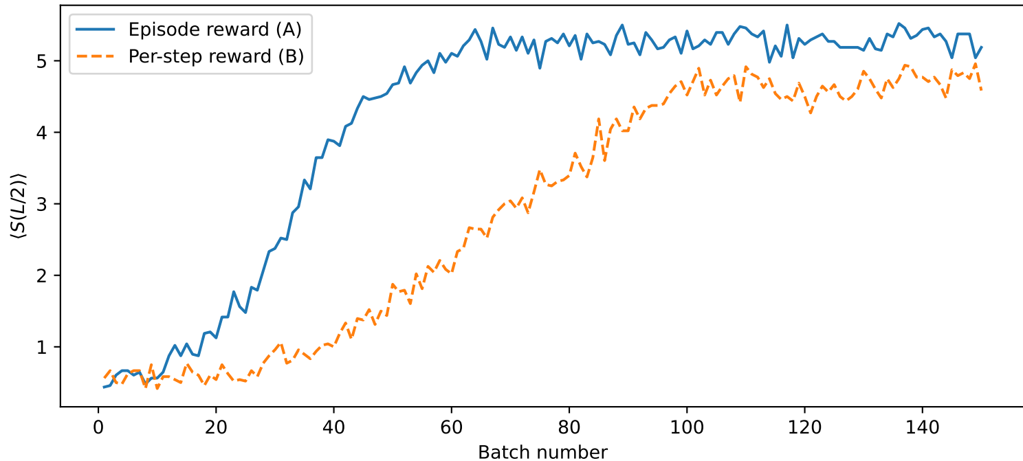
Training curves — L = 24 , k = 8 : episode vs per-step reward
