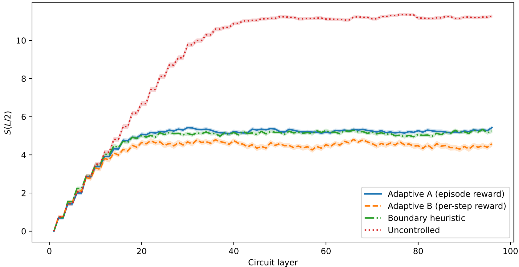
Entropy trajectory — L = 24 , k = 8 : episode vs per-step reward
