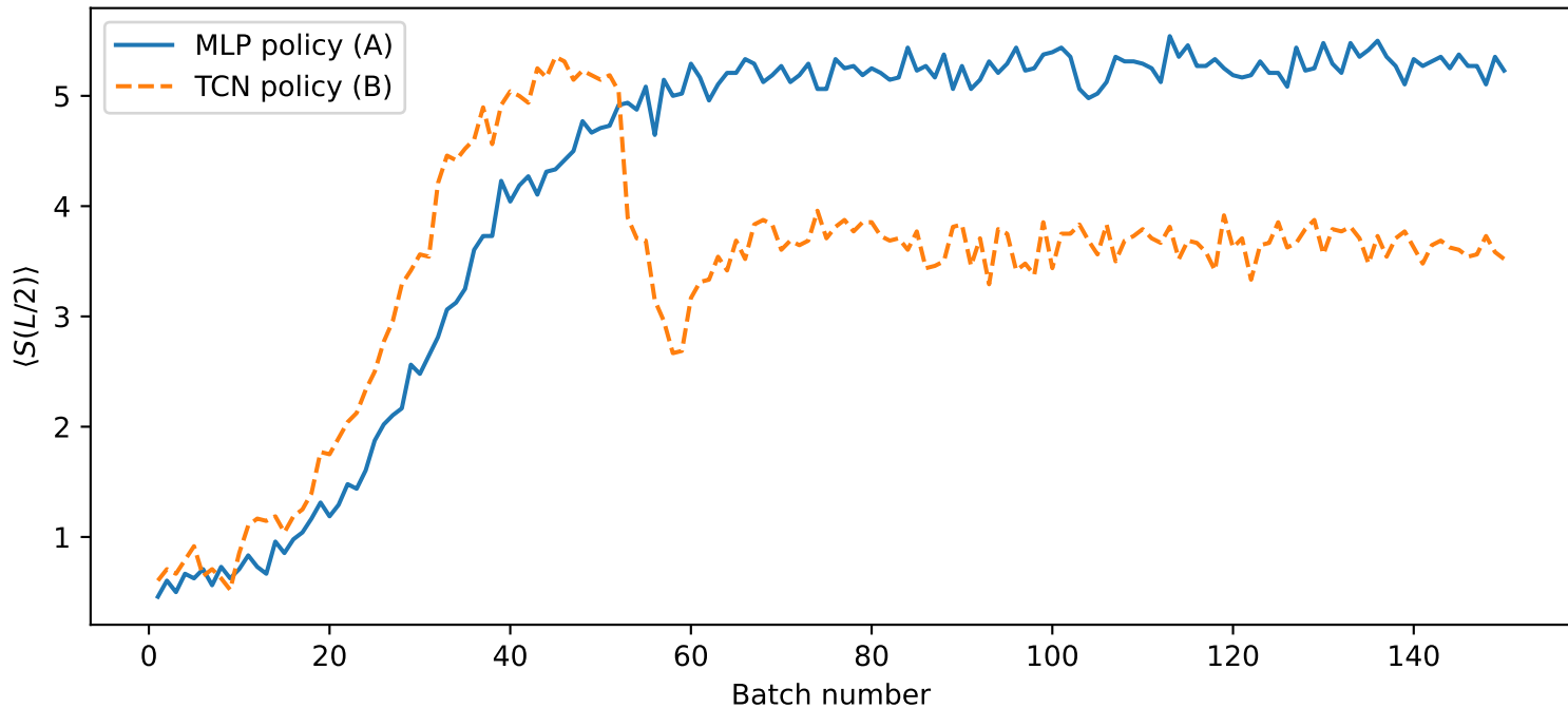
Training curves — L = 24, k = 8 : MLP vs TCN policy
