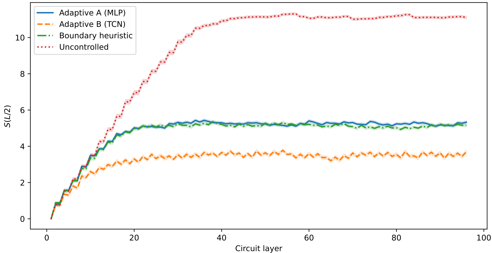
Entropy trajectory — L = 24, k = 8 : MLP vs TCN policy
