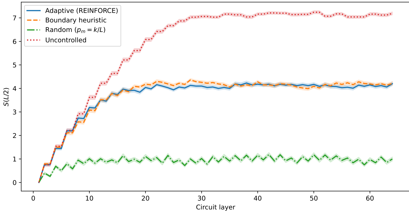
Entropy trajectory — L = 16, k = 3, 100 episodes
