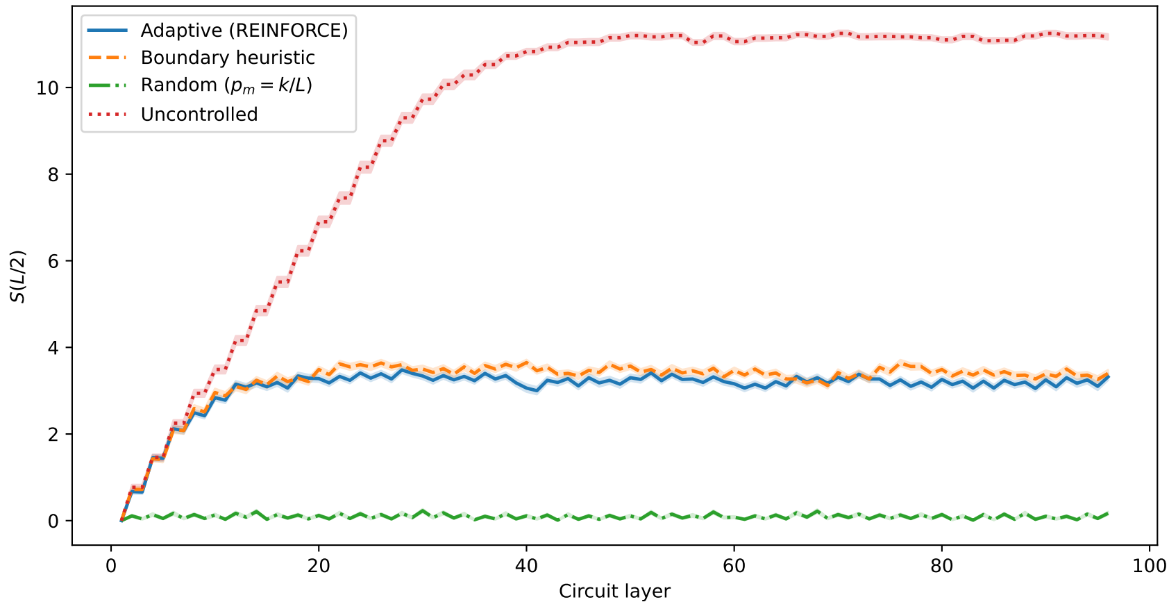
Entropy trajectory — L = 24, k = 12, 100 episodes
