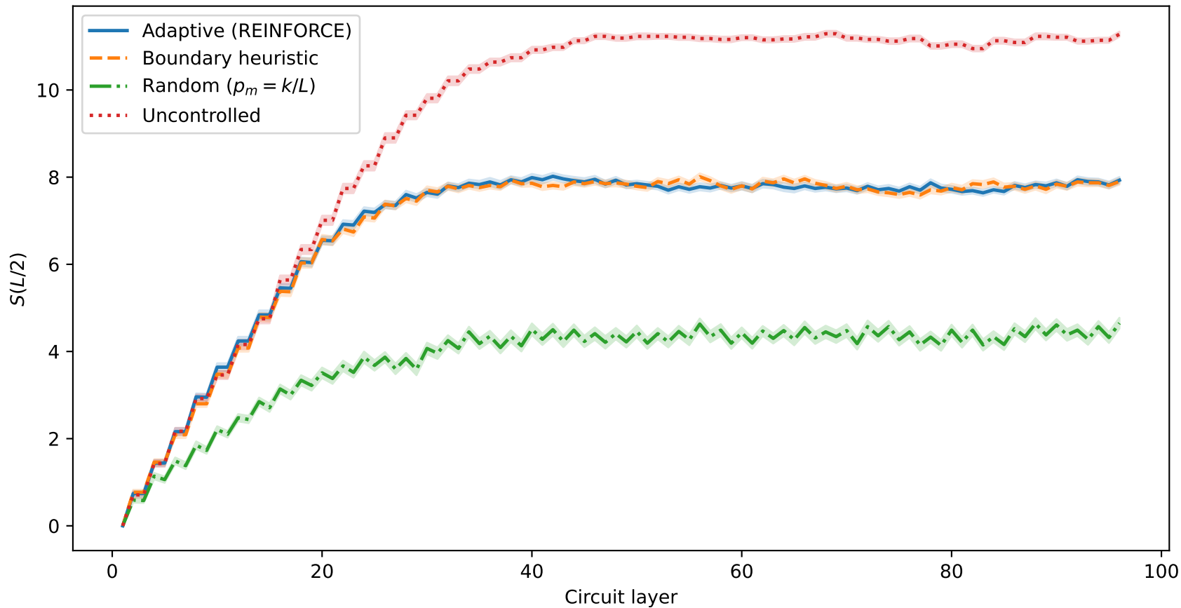
Entropy trajectory — L = 24 , k = 2 , 100 episodes
