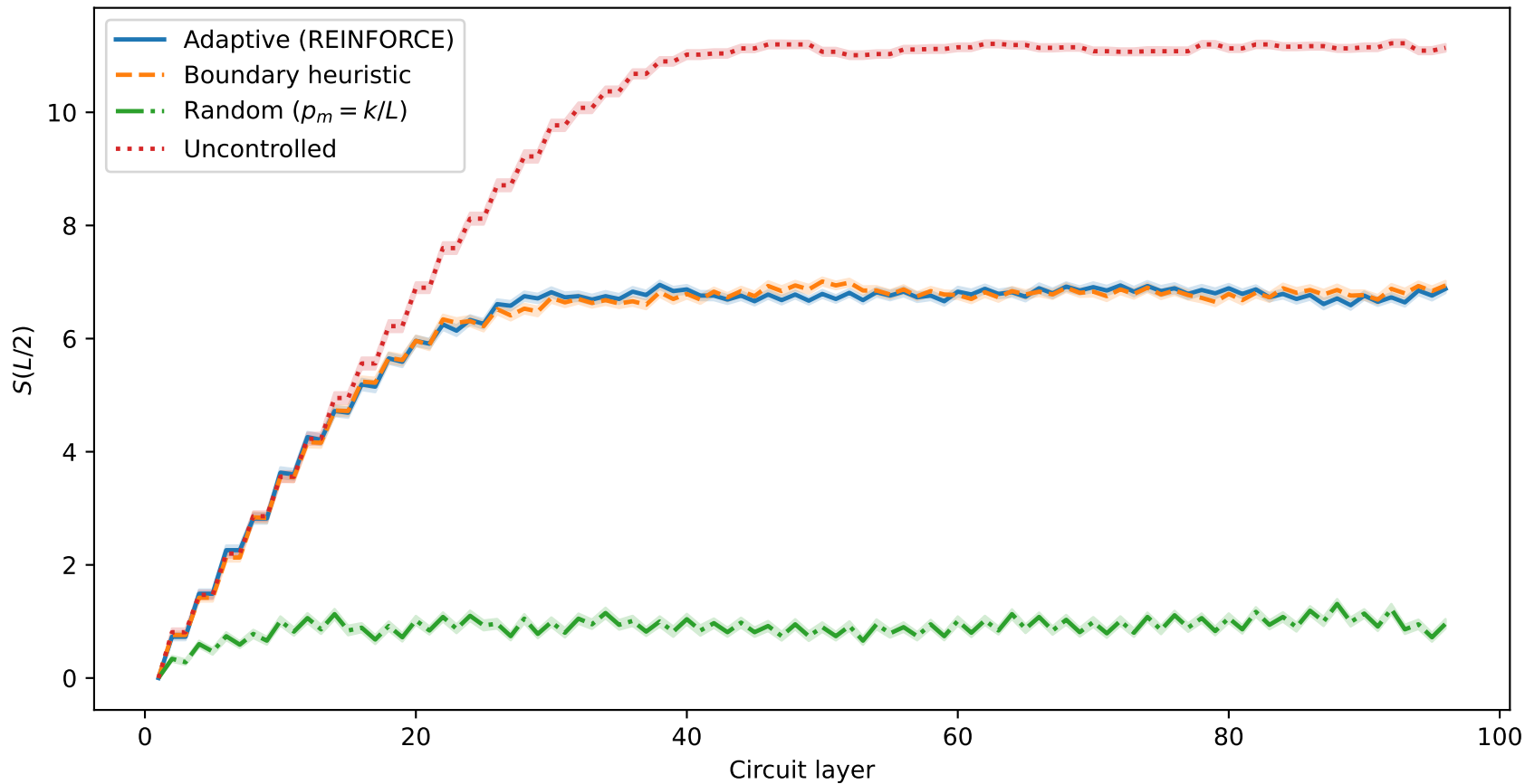
Entropy trajectory — L = 24 , k = 5 , 100 episodes
