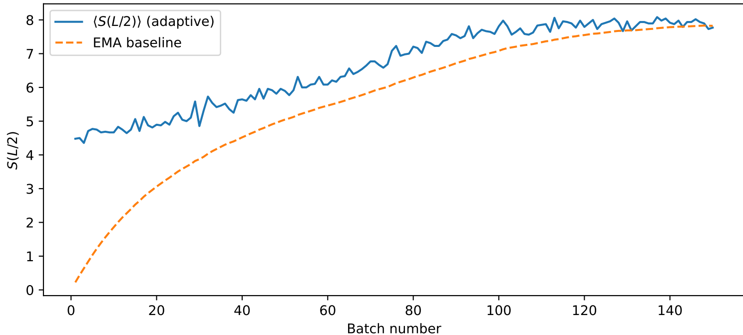
REINFORCE training curve — L = 24, k = 2
