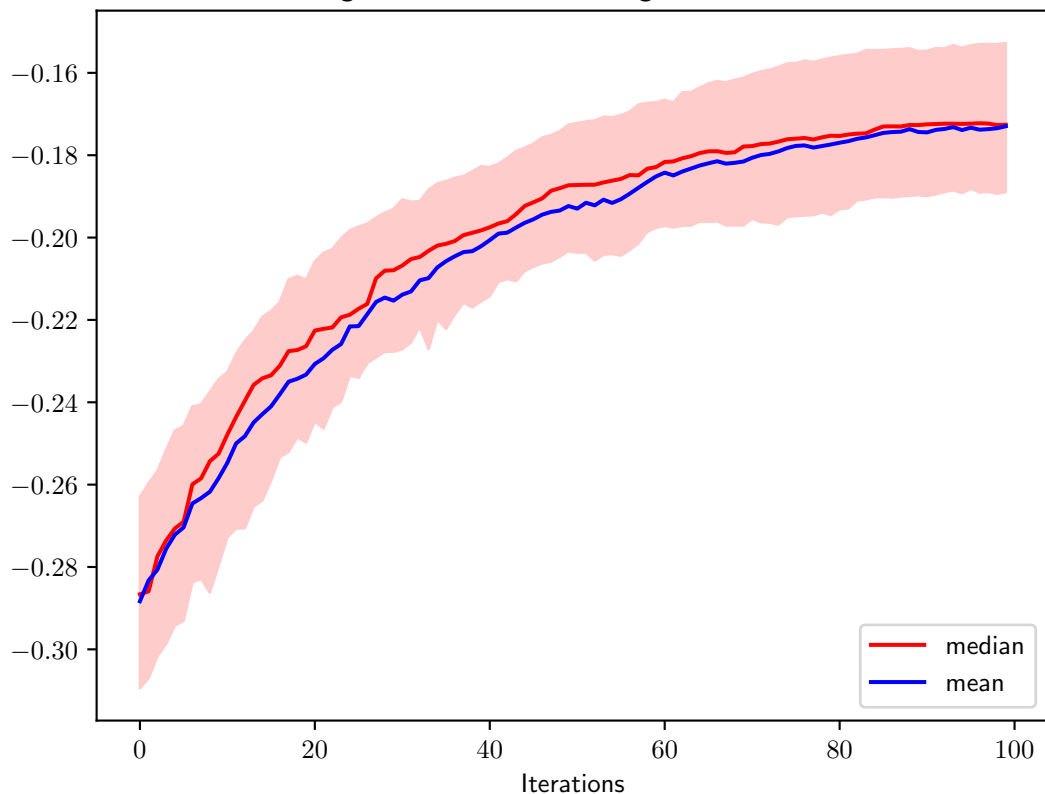
Convergence of the CSPSA algorithm for \alpha = 0.4
