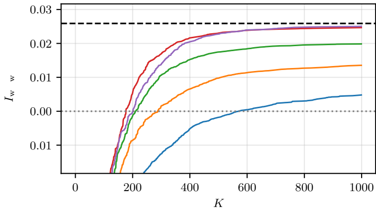
Schmidt states
