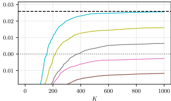
Werner states
