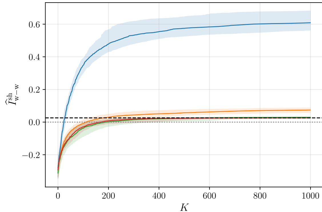
Full Classical Shadows
