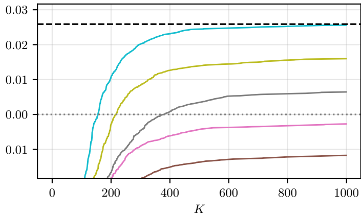
Werner states
