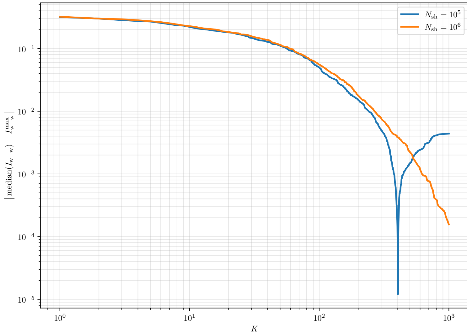
Sim01_02 — Distance to the quantum maximum, N_{\text{sh}} = 10^5 vs 10^6
