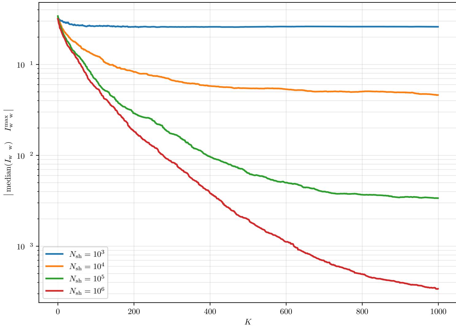
Sim01_04 — Distance to the quantum maximum, Mix, by N_{\text{sh}}
