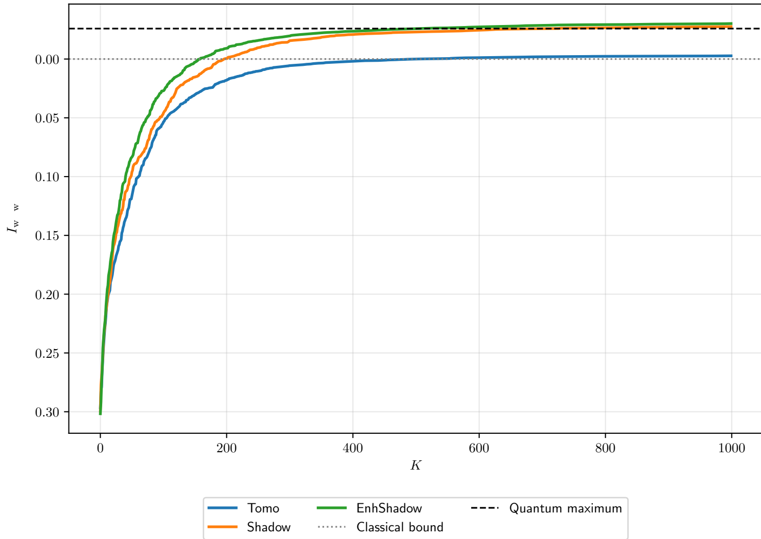
Simulation 01 — Median convergence, maximally entangled state
