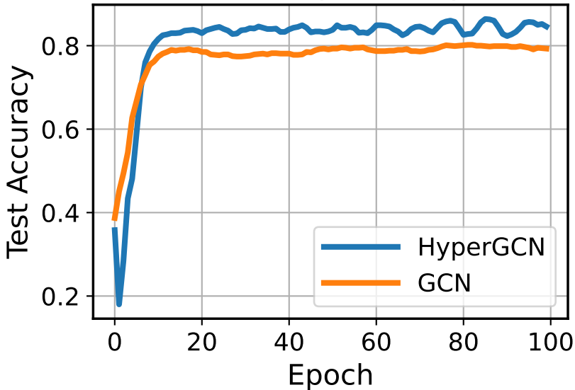
Test Accuracy over Epochs
