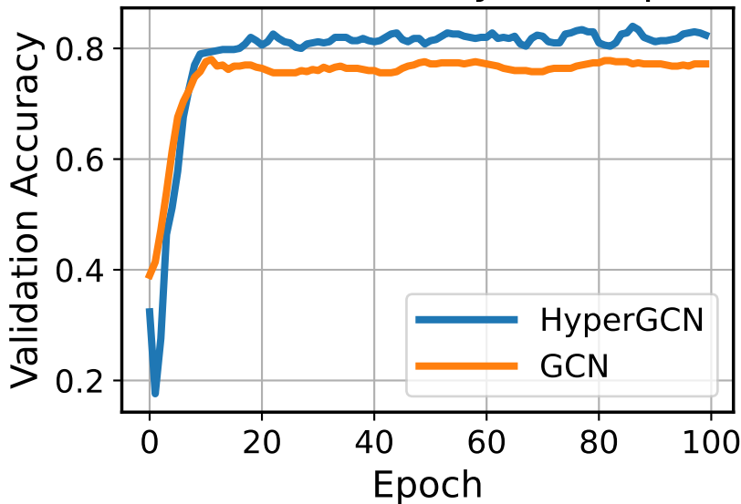
Validation Accuracy over Epochs
