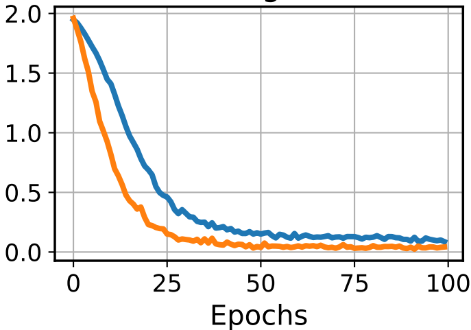
Training Loss
