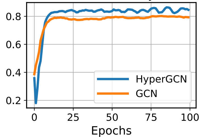
Test Accuracy
