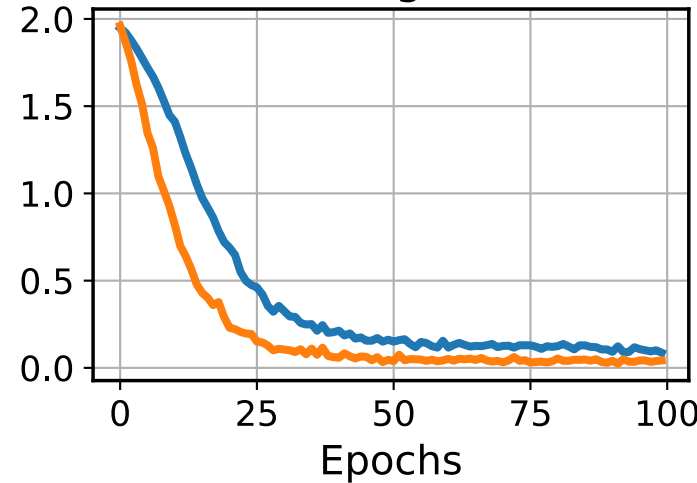
Training Loss
