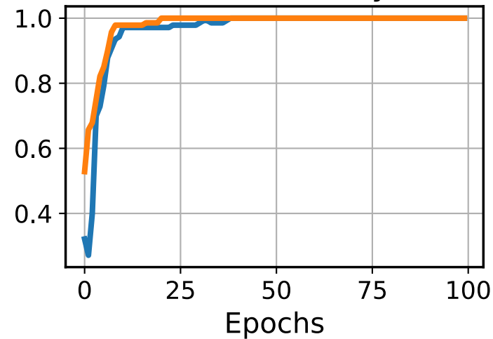
Train Accuracy
