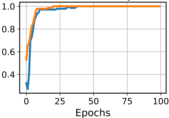
Train Accuracy
