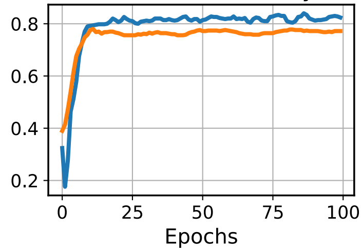
Validation Accuracy
