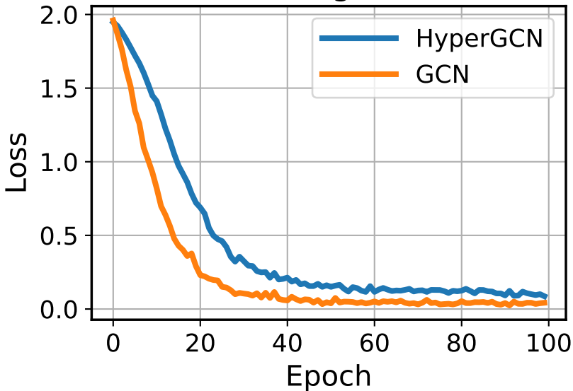
Training Loss
