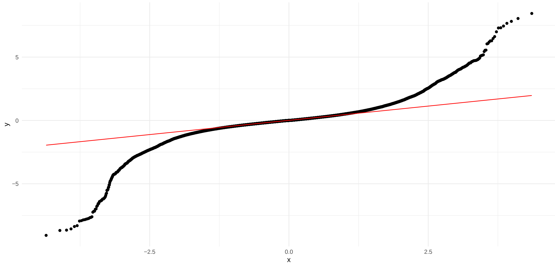
QQ-Plot: All Proteins Distribution
