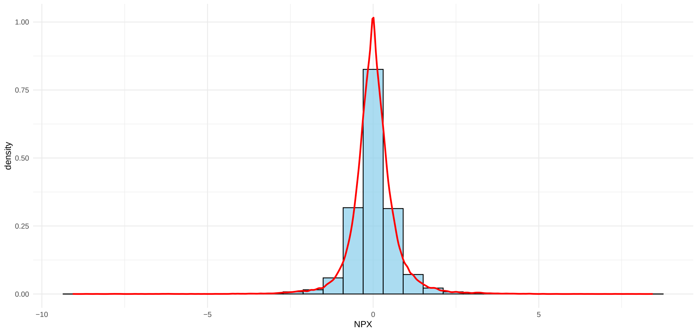
Histogram: All Proteins Distribution
