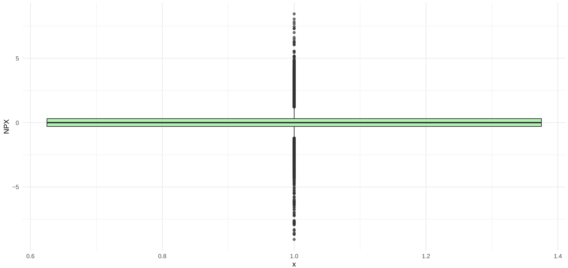
Boxplot: All Proteins Distribution
