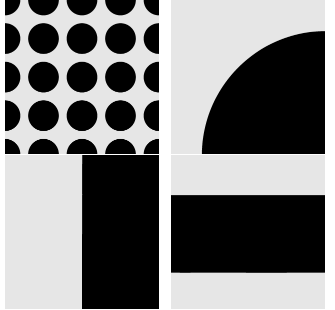
Figure 13: Examples of resource allocation optimization in population dynamics. Initial guess (top-left) and optimized designs for r = 10 (top-right), r = 40 (bottom-left), and r = 100 (bottom-right). The stopping criterion was satisfied at 147, 107, and 167 iterations, respectively.
