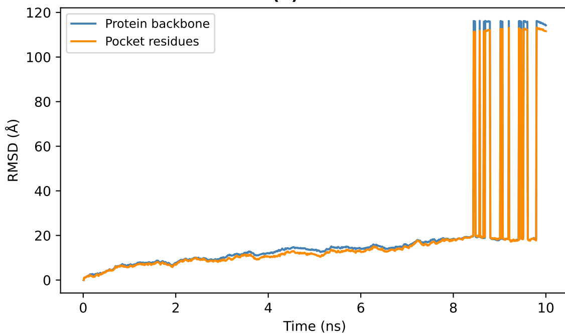
(C) RMSD
