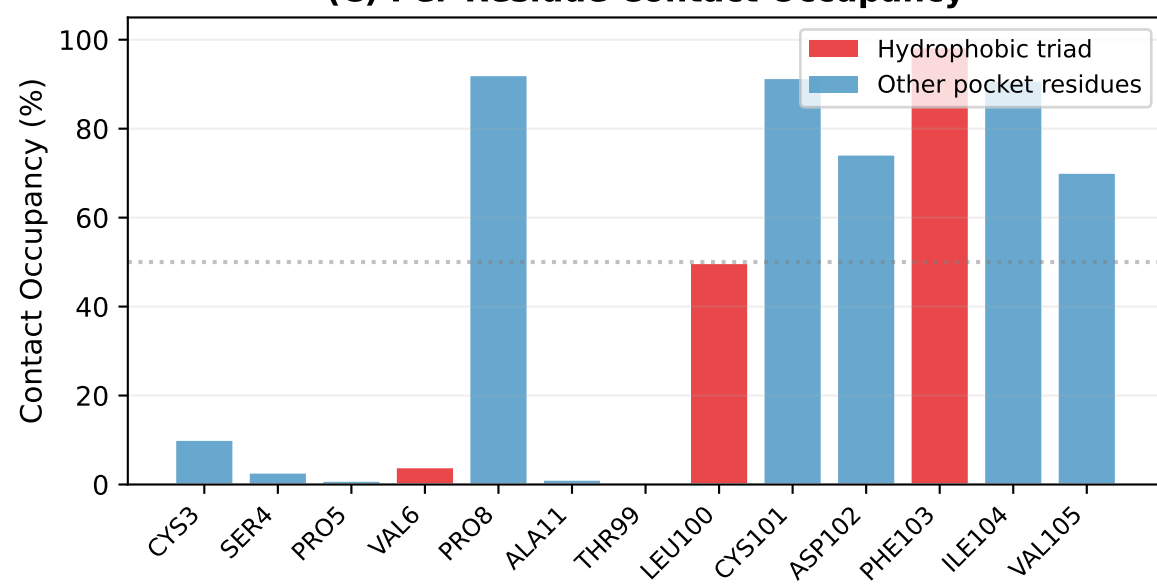
(C) Per-Residue Contact Occupancy
