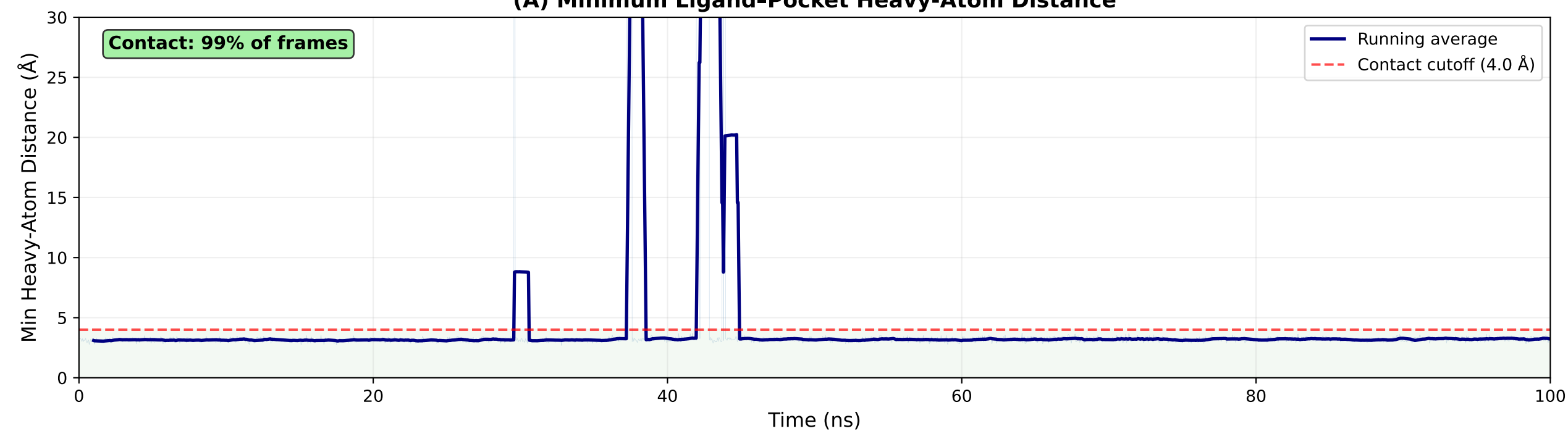
(A) Minimum Ligand-Pocket Heavy-Atom Distance
