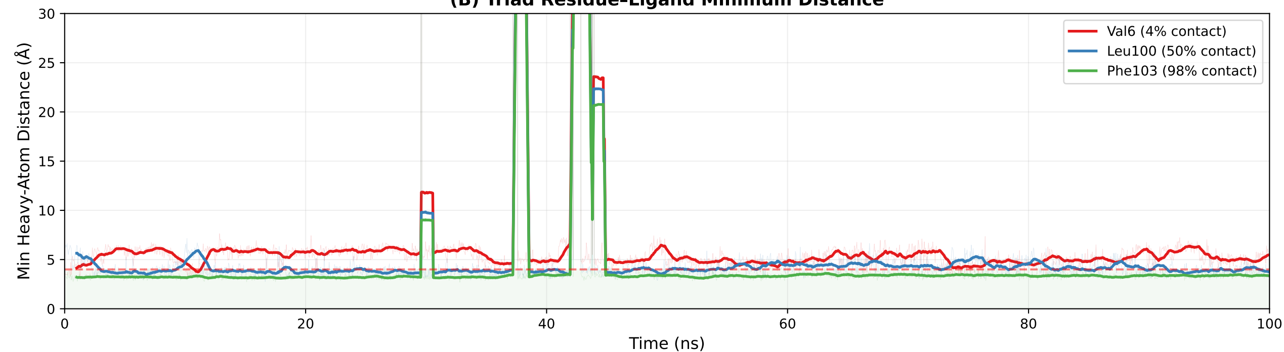
(B) Triad Residue-Ligand Minimum Distance
